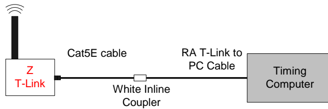
Figure 9: Basic Connection with a 50' extension, Wiring Diagram
